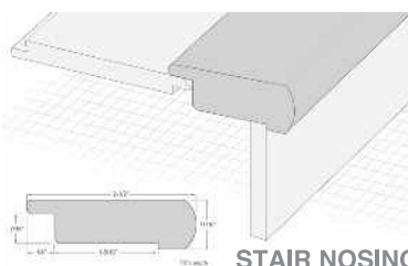
STAIR NOSING
